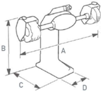
Twin shaft buffering polishing machine with self ventilated disk
